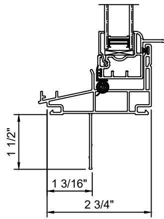
V100/V150 Hung
