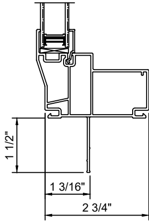
V100/V150 Fixed
