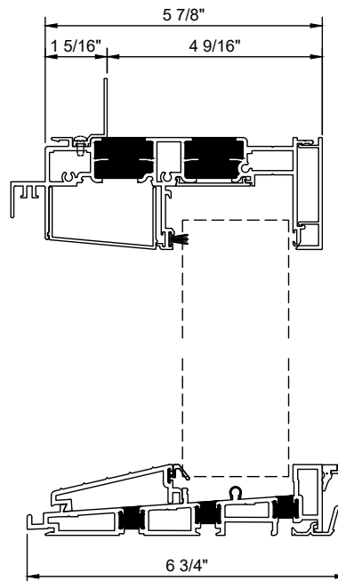
Low Profile Sill Operable Side
