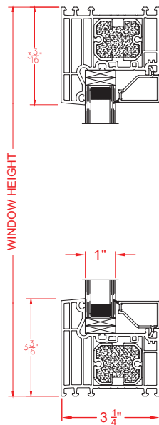
Fixed
