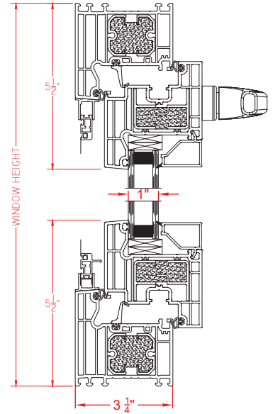
Project-In Hopper
