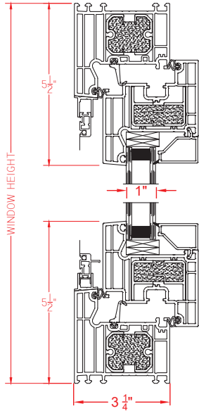
Project-In Casement
