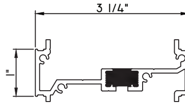
1" STACK MULL
