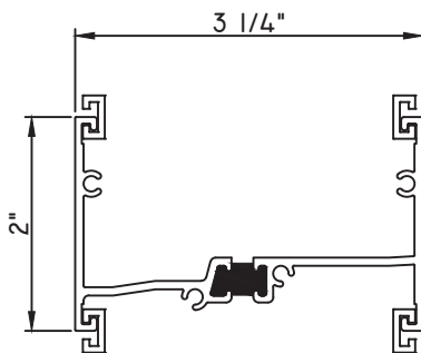
2" STACK MULL
