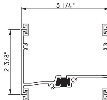
2 3/8" STACK MULL
