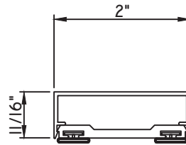
2" MULL COVER MAX17386 - BASE M23502 - CAP BPN-9159 - W.S. (QTY. 2)
