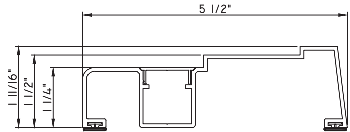
5 1/2" MULL COVER M23979 - MULL COVER M536207 - CAP BPN-9159 - W.S. (QTY. 2)
