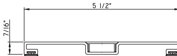
5 1/2" MULL COVER M536206 - MULL COVER M536207 - CAP BPN-9159 - W.S. (QTY. 2)
