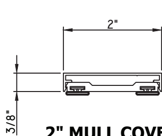
2" MULL COVER MAX17386 - BASE MAX14141 - CAP BPN-9159 - W.S. (QTY. 2)
