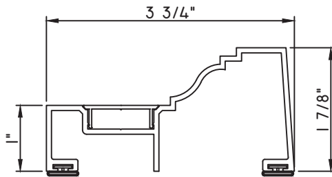
3 3/4" MULL COVER M24837 - MULL COVER M536207 - CAP BPN-9159 - W.S. (QTY. 2)
