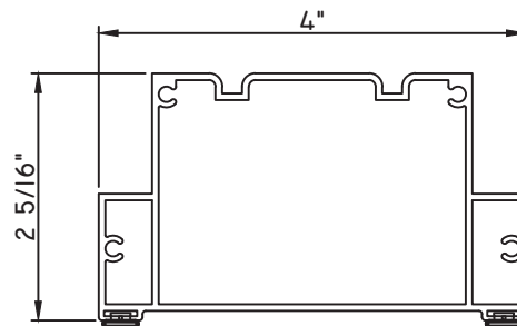
4" MULL COVER M24428 - MULL COVER BPN-9159 - W.S. (QTY. 2) MH8-18X1 LP - SCREW (QTY. 8)
