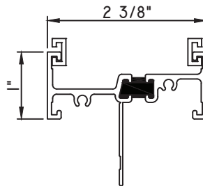
1" STACK MULL M43325 - STACK MULL QWP-43325 - END DAMS (QTY. 2) MH8-18X1 LP - SCREW (QTY. 4) 970-300 - WEEP COVER
