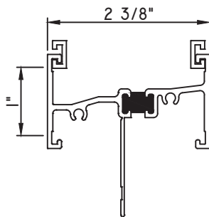
1 3/8" STACK MULL MW23712 - STACK MULL QWP-070706 - END DAMS (QTY. 2) MH8-18X1 LP - SCREW (QTY. 4) 970-300 - WEEP COVER
