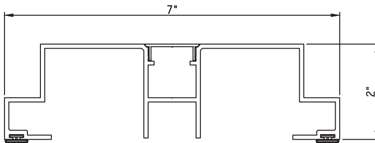
7" MULL COVER M25907 - MULL COVER M536207 - CAP BPN-9159 - W.S. (QTY. 2)
