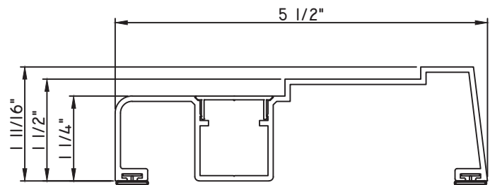
5 1/2" MULL COVER M23979 - MULL COVER M536207 - CAP BPN-9159 - W.S. (QTY. 2)
