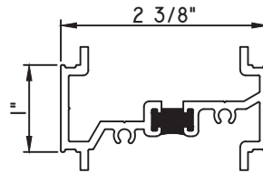
1" STACK MULL MW25615 - STACK MULL 970-300 - WEEP COVER MH8-18X1 LP - SCREW (QTY. 4)
