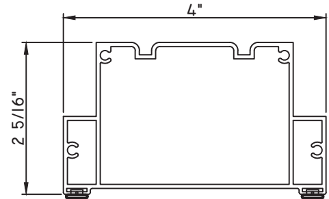
4" MULL COVER M24428 - MULL COVER BPN-9159 - W.S. (QTY. 2) MH8-18X1 LP - SCREW (QTY. 8)
