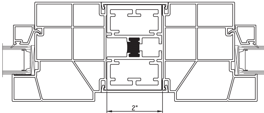
2" MULLION M22784 - MULL MULL CAP: M22941 C-MULL: D315 (WHITE) SD315 (SANDSTONE)
