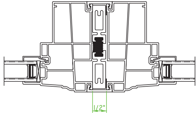
1/2" MULL M20427 - MULL MULL CAP: D317 (WHITE)
