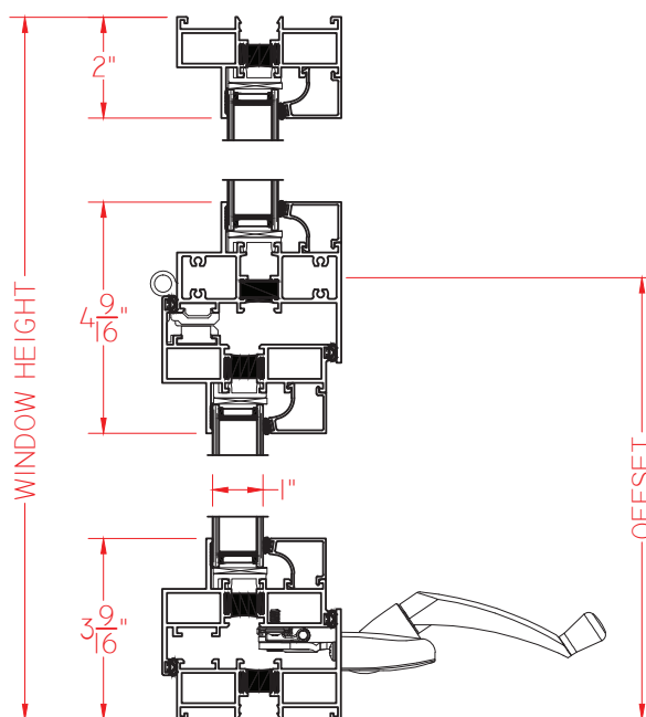
Ⓐ VERTICAL CROSS SECTION
