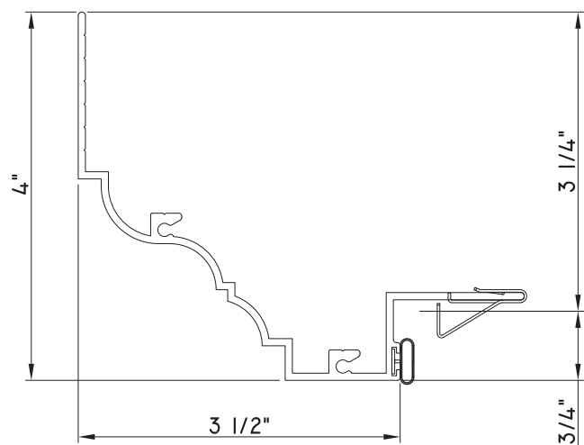
PRESET PANNING M26033 - PANNING BPN-9159 - W.S. MH8-18X1 LP - FASTENER (QTY. 8) 1974 - CLIP (6" FROM EACH CORNER & 20" O.C.)
