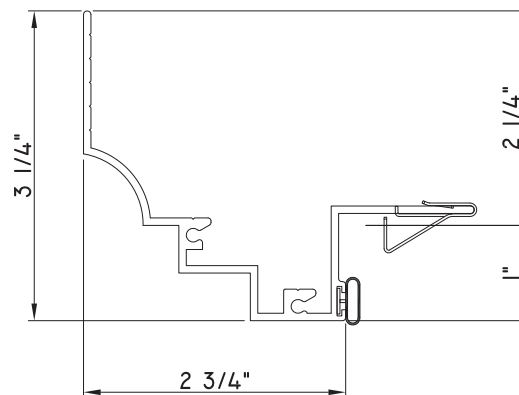
PRESET PANNING M25598 - PANNING BPN-9159 - W.S. MH8-18X1 LP - FASTENER (QTY. 8) 1974 - CLIP (6" FROM EACH CORNER & 20" O.C.)
