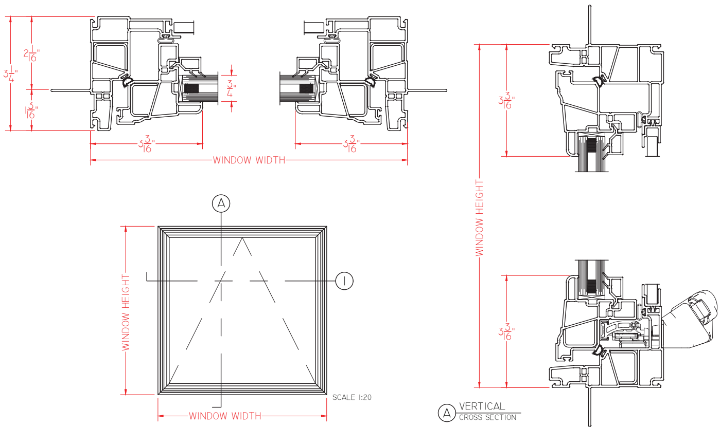
① HORIZONTAL CROSS SECTION
