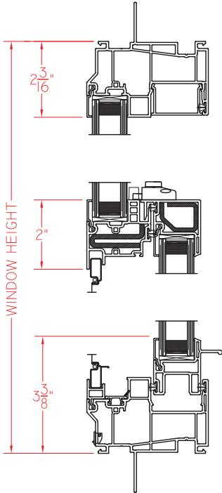
Single Hung (CW50)
