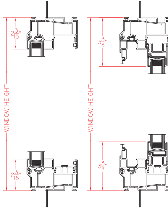
Horizontal Slider (CW50)
