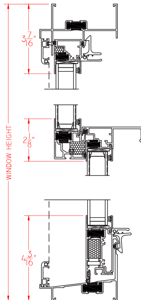
A VERTICAL CROSS SECTION
