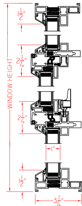
Floating Operator
