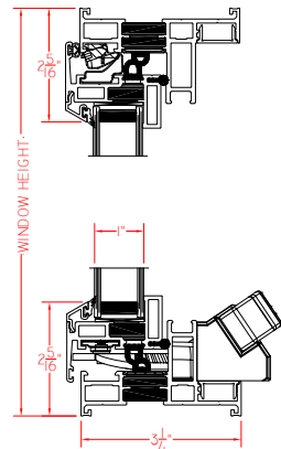
Project-Out Roto
