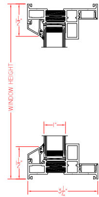
Fixed
