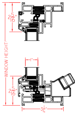
Casement Roto
