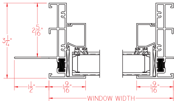
① HORIZONTAL CROSS SECTION
