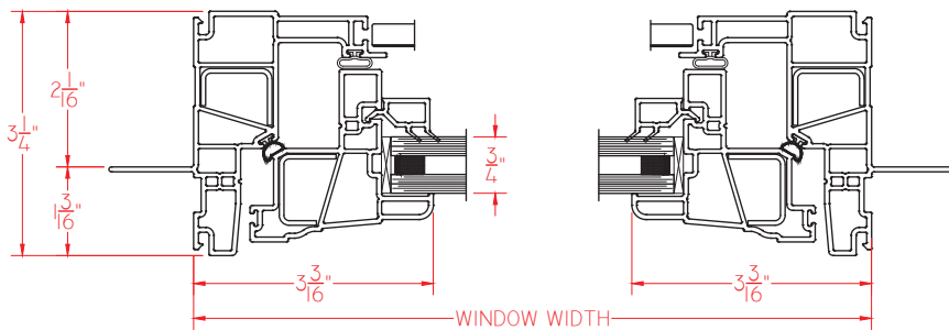
① HORIZONTAL CROSS SECTION
