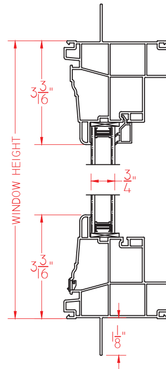
Ⓐ VERTICAL CROSS SECTION
