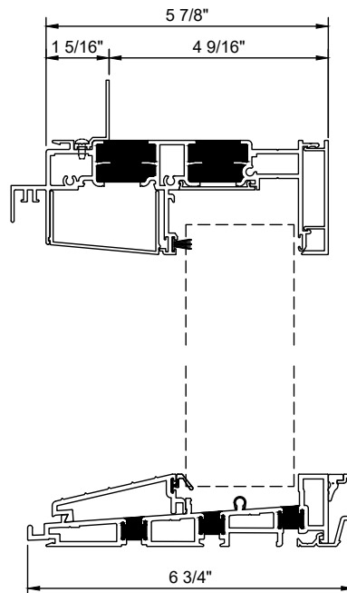
Low Profile Sill Operable Side
