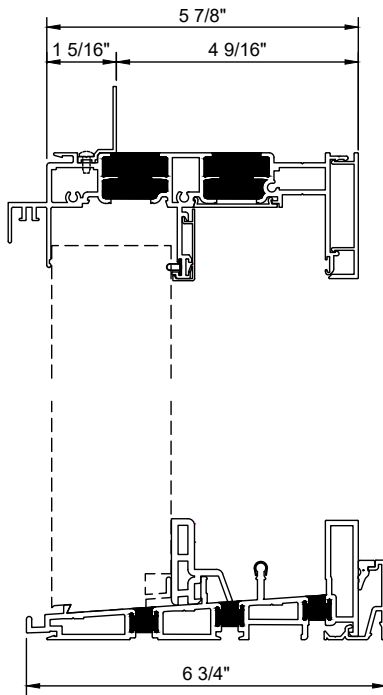
Standard Sill Fixed Side
