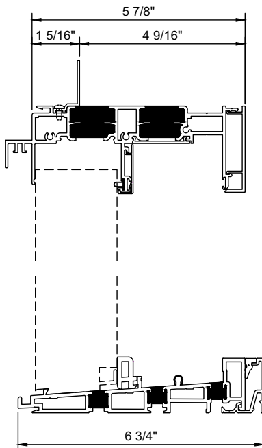
Low Profile Sill Fixed Side
