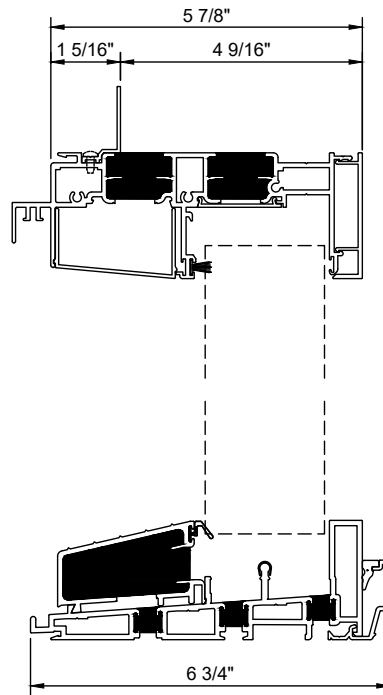
Standard Sill Operable Side
