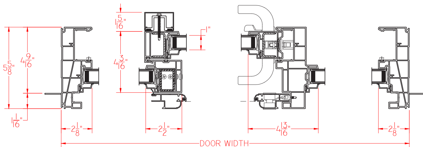
I HORIZONTAL CROSS SECTION
