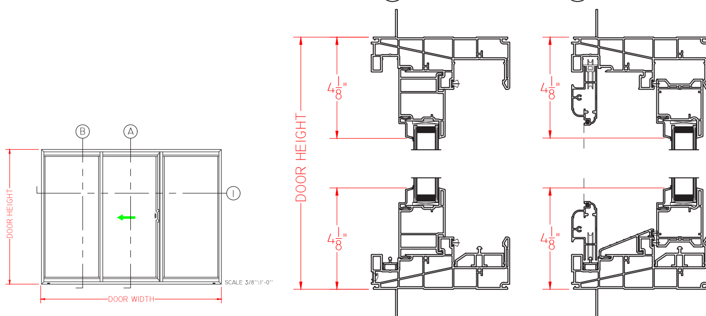
B VERTICAL CROSS SECTION
