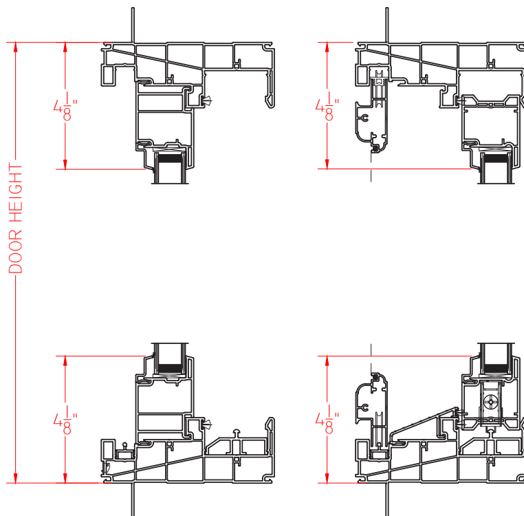
② VERTICAL CROSS SECTION
